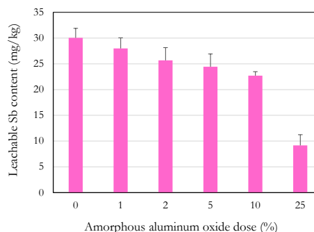
Fig 2. Leaching behavior of treated mine waste rocks.
