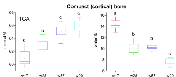
Fig 1. TG analyses: mineral (left) and water (right) content (%) in hen tibiae bone samples as a function of age (17-90 weeks).
