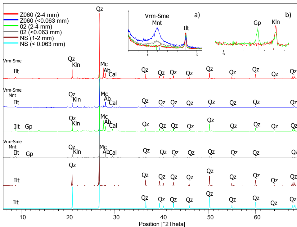
Fig 1. Analysis of the majority mineral phases by X-ray diffraction for samples <0.063 and 2-4 of materials Z060 and 02, and for NS samples <0.063 and 1-2 mm. a) Detail of the phyllosilicate phases. b) Detail of the gypsum phase and kaolinite phase. (Ab - Albite, Cal - Calcite, Gp - Gypsum, Ilt - Illite, Kln - Kaolinite, Mc - Microcline, Mnt - Montmorillonite, Qz - Quartz, Sme - Esmeclite, Vrm - Vermiculite).
