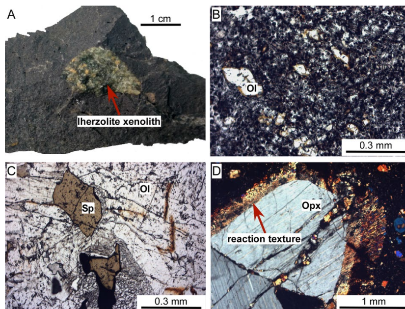
Fig 1. (A) spinel lherzolite in volcanic rock; (B) olivine crystals in a glassy groundmass containing opaque minerals and olivine microcrystals partially altered by iddingsite; (C) spinel grains included in the xenolith; (D) pyroxene-rich corona in lherzolite xenolith.
