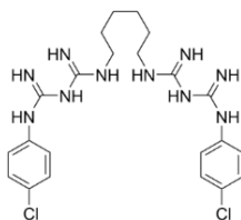
Fig. 1. Chemical structure of chlorhexidine
