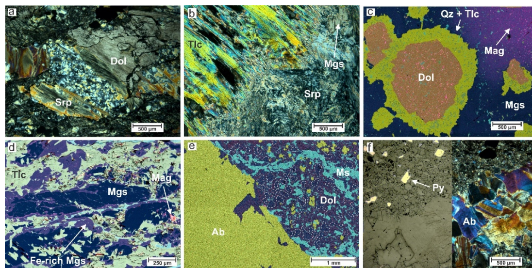
Fig 1. Replacement and dissolution–precipitation structures in samples of the Point-Rousse ophiolite. a) Bastite texture composed of serpentine (Srp) replaced by dolomite (Dol). b) Serpentine in foliated serpentinite replaced by large crystals of talc (Tlc) and magnesite (Mgs). c) EDS-SEM false-colour phase map of a corona-shaped reaction rim of quartz (Qz) and talc (Tlc) around rounded dolomite, and coarse-grained magnesite chemically zoned (reddish area) with magnetite (Mag) inclusions. d) EDS-SEM false-colour phase map of deformed magnesite with Fe-content zoning. e) EDS-SEM false-colour phase map of massive albite–carbonate rock composed of zoned dolomite (white dashed lines), albite (Ab) and muscovite (Ms) crosscut by albite vein. f) Pyrite (Py) in carbonated green-schist related to albite vein.
